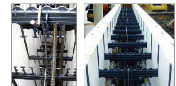
Vertical & Horizontal Clips in place close to corner Showing HV Clips holding down a top row that has been cut down to +/- 8" in height
