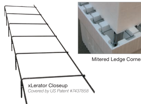
Ledge Form with xLerator
