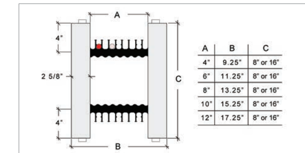
Fox Blocks 90° Extended Corner Size Chart
