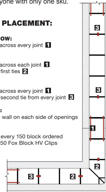
Vertical Clips in Place Horizontal Clips in Place Note: You can skew the HV Clip a notch or two for an even tighter fit, if needed.
