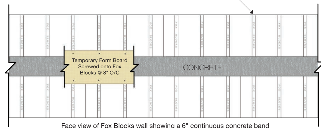
Face view of Fox Blocks wall showing a 6" continuous concrete band
